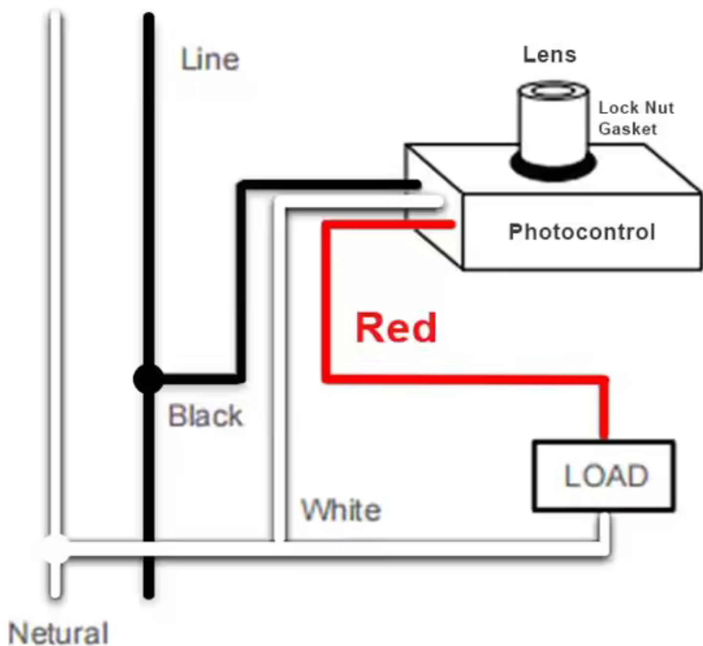
3-way Wiring Mounting Diagram
